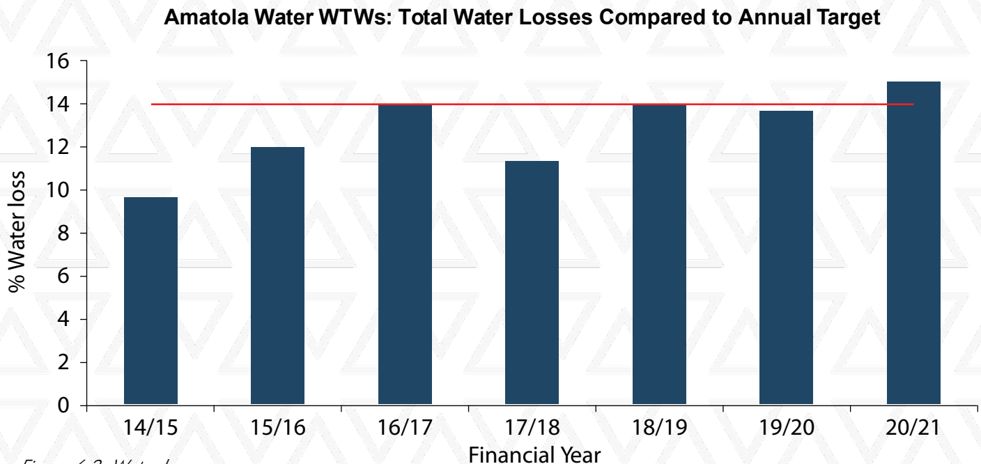
Figure 6.3: Water losses
