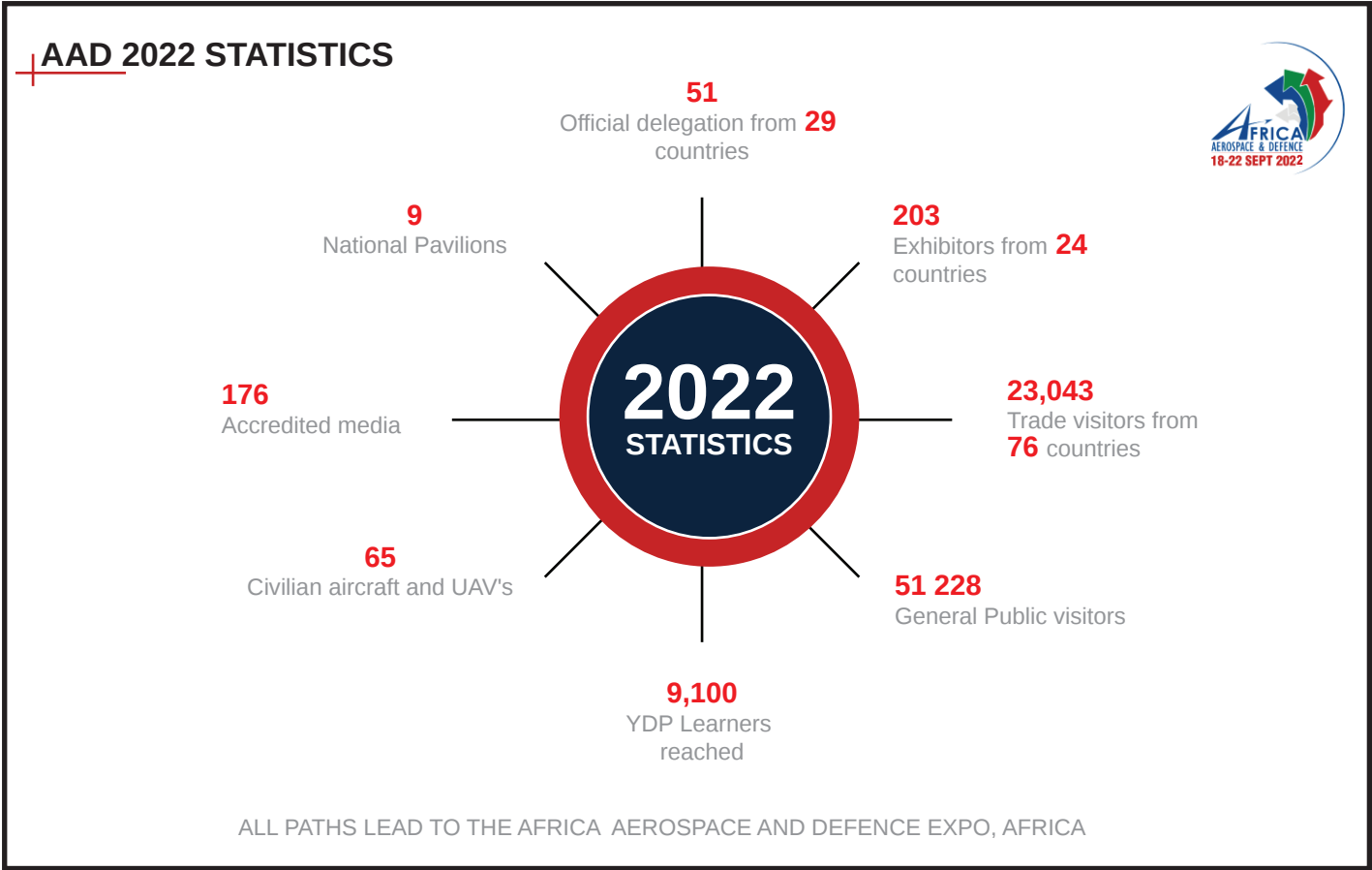
Figure 25: AAD 2022 STATISTICS
