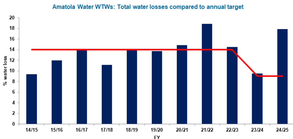
Figure 7.2: Amatola Water, water treatment works (WTWs): Total water losses compared to the annual target
